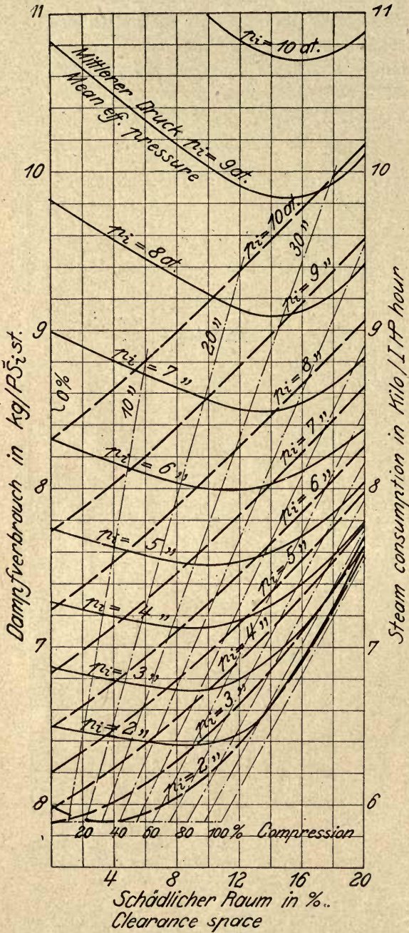
Fig. 19. Saturated steam 14 at. abs. Noncondensing.
