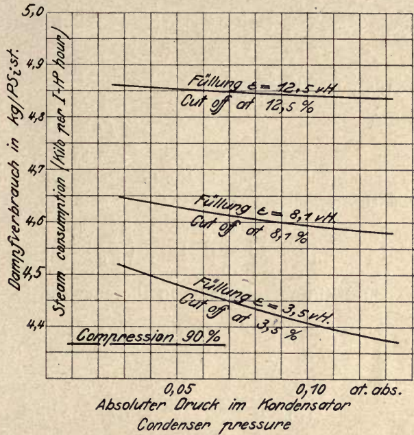
Fig. 31. Superheated steam 300° C, 13 at. abs. Clearance space 5%.
