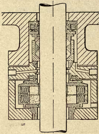
Type B Duplex packing for steam pressures above 6 at. and condensing service.
