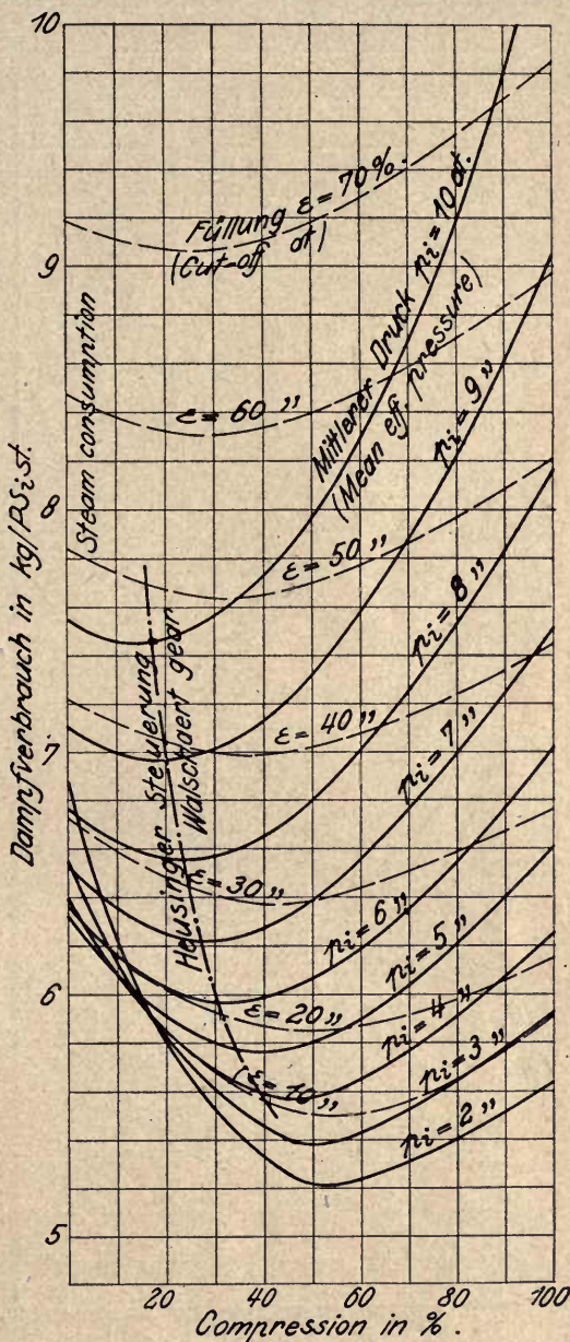
Fig. 14. Superheated steam 300° C, 14 at. abs. Noncondensing, Clearance space 8%.
