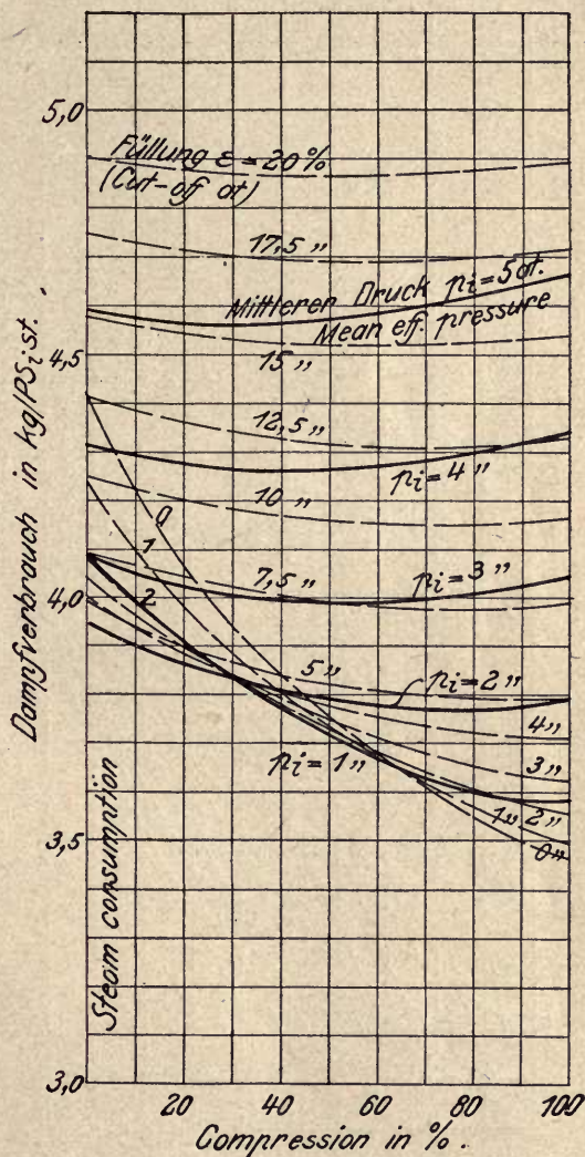
Fig. 18. Superheated steam 300° C, 14 at. abs. Condensing (0.08 at. abs.) Clearance space 2 %.
