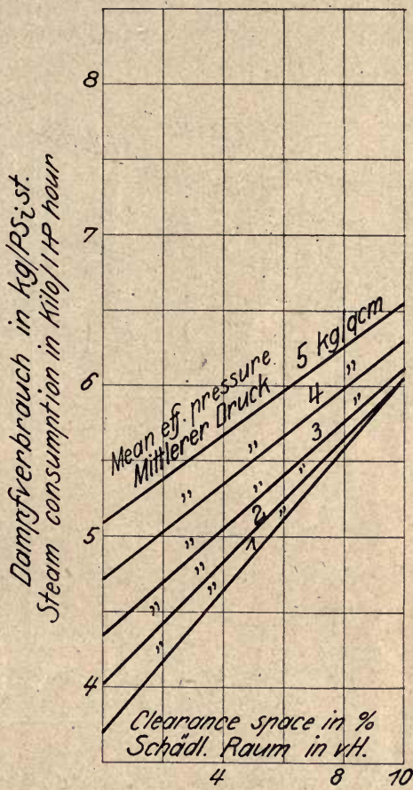
Fig. 22. Saturated steam 13 at. abs. Condensing (0.1 at. abs.). Most favourable compression.
