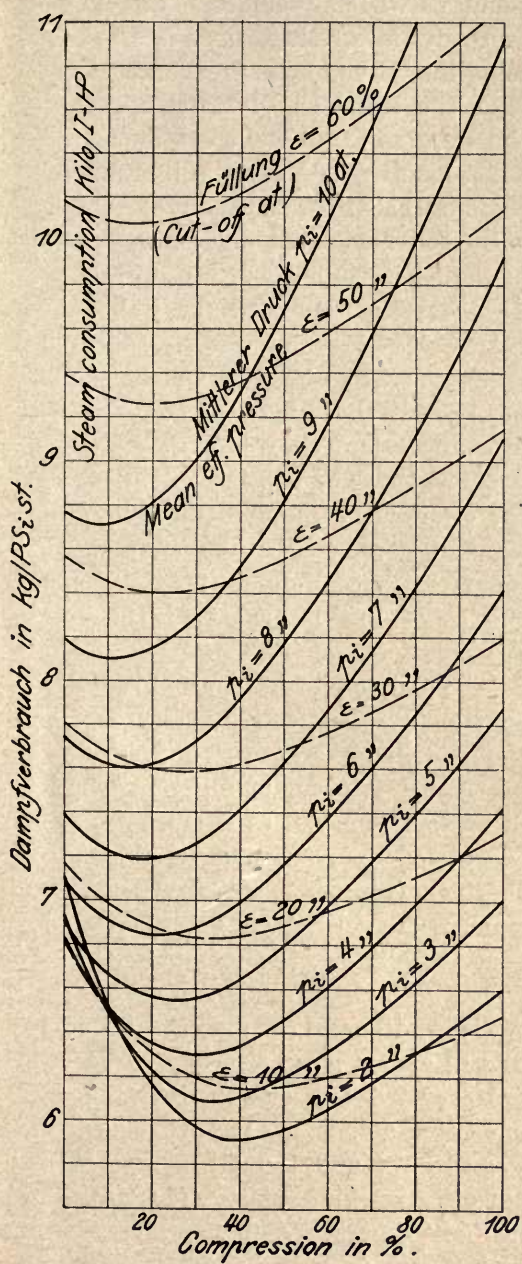
Fig. 10. Saturated steam 14 at. abs. Noncondensing, Clearance space 5%.
