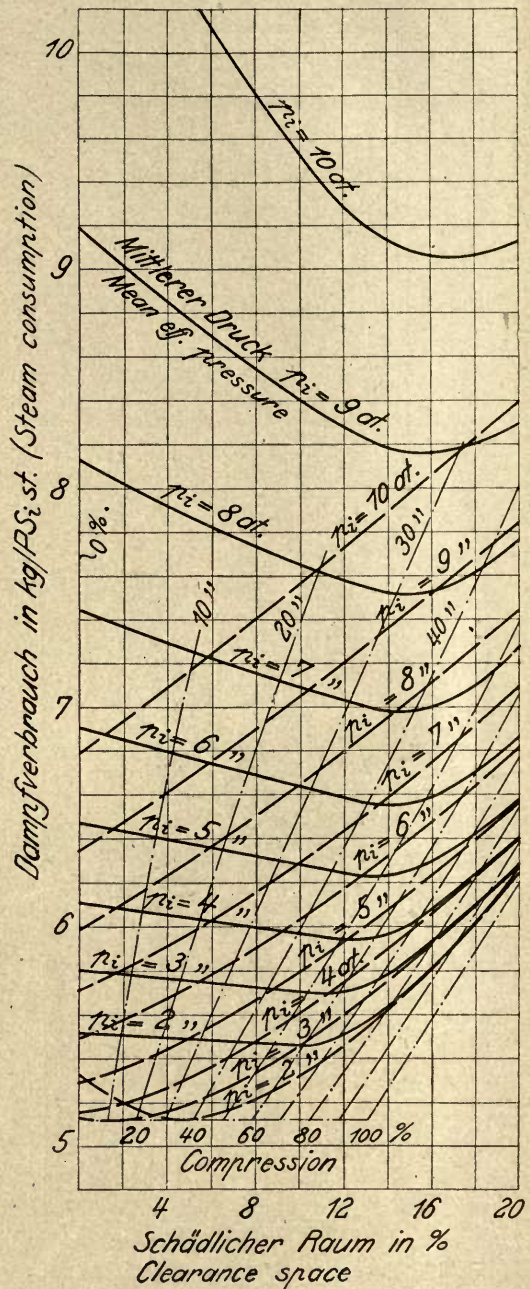
Fig. 20. Superheated steam 300° C, 14 at. abs. Noncondensing.
