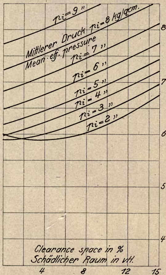
Fig. 21. Saturated steam 13 at. abs. Noncondensing. Most favourable compression.
