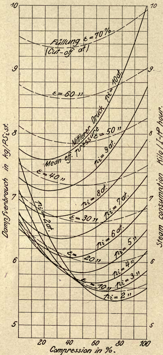
Fig. 15. Superheated steam 300° C, 14 at. abs. Noncondensing, Clearance space 11%.
