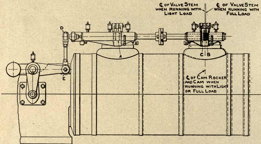
Fig. 54. Sectional View of Expansion-Compensating Gear.
