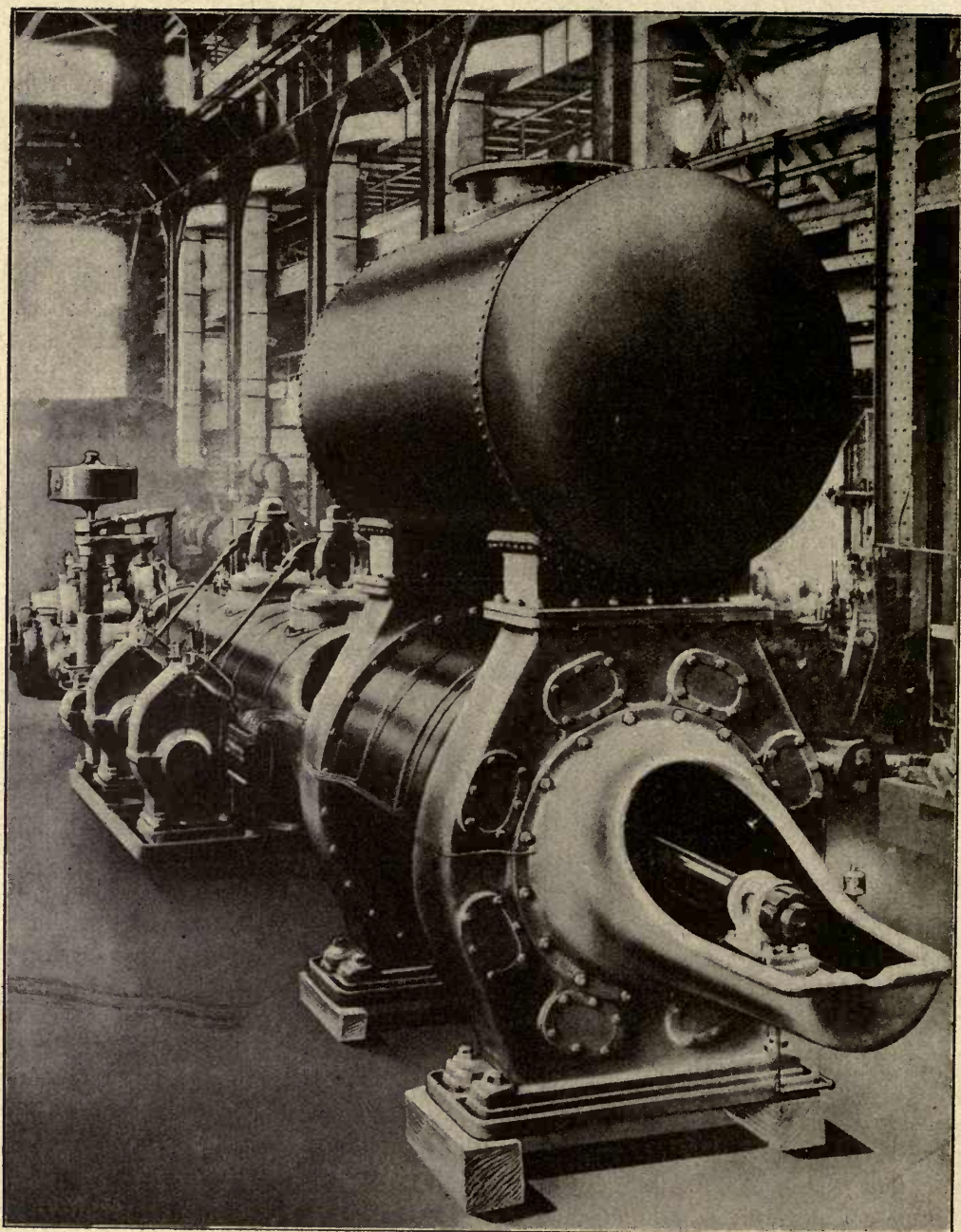
Fig. 11. Una-Flow Blowing Engine built by the Mesta Machine Company Pittsburgh.
