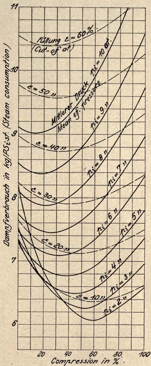
Fig. 11. Saturated steam 14 at. abs. Noncondensing, Clearance space 8%.
