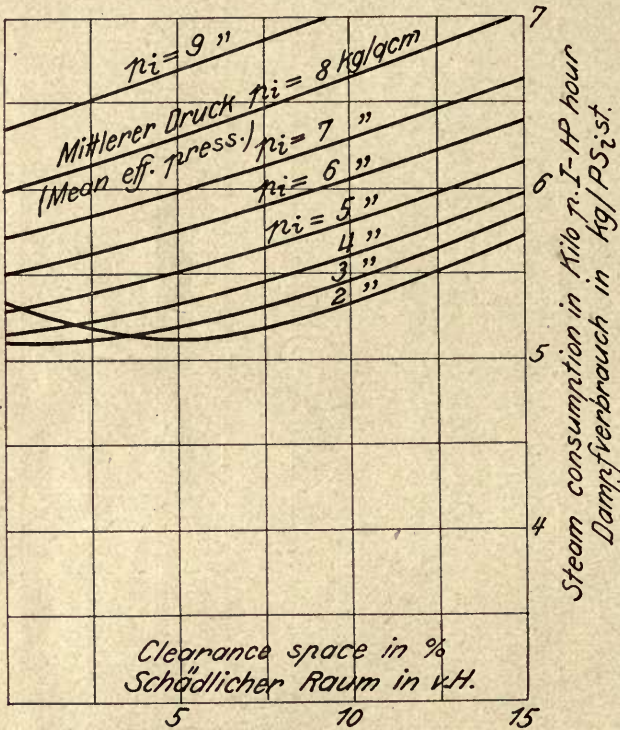
Fig. 23. Superheated steam 300° C, 13 at. abs. Noncondensing. Most favourable compression.
