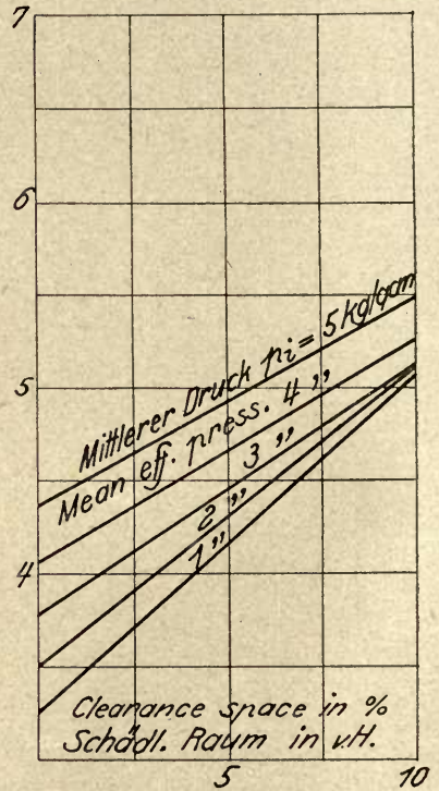
Fig. 24. Superheated steam 300° C, 13 at. abs. Condensing (0.1 at. abs.) Most favourable compression.
