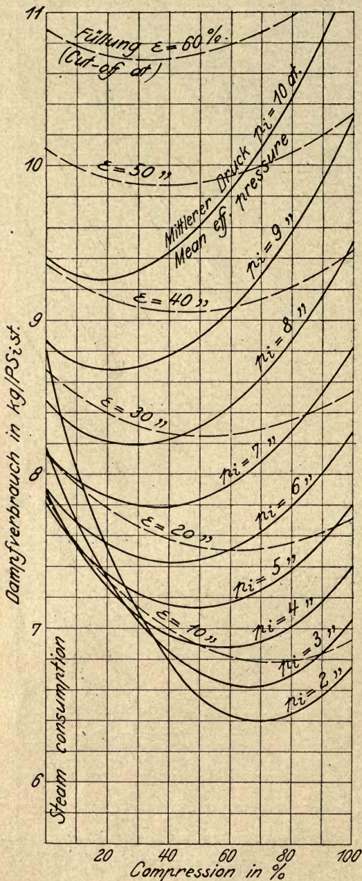
Fig. 12. Saturated steam 14 at. abs. Noncondensing, Clearance space 11%.
