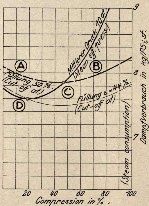
Fig. 17. Superheated steam 300° C, 14 at. abs. Noncondensing, Clearance space 11 %.
