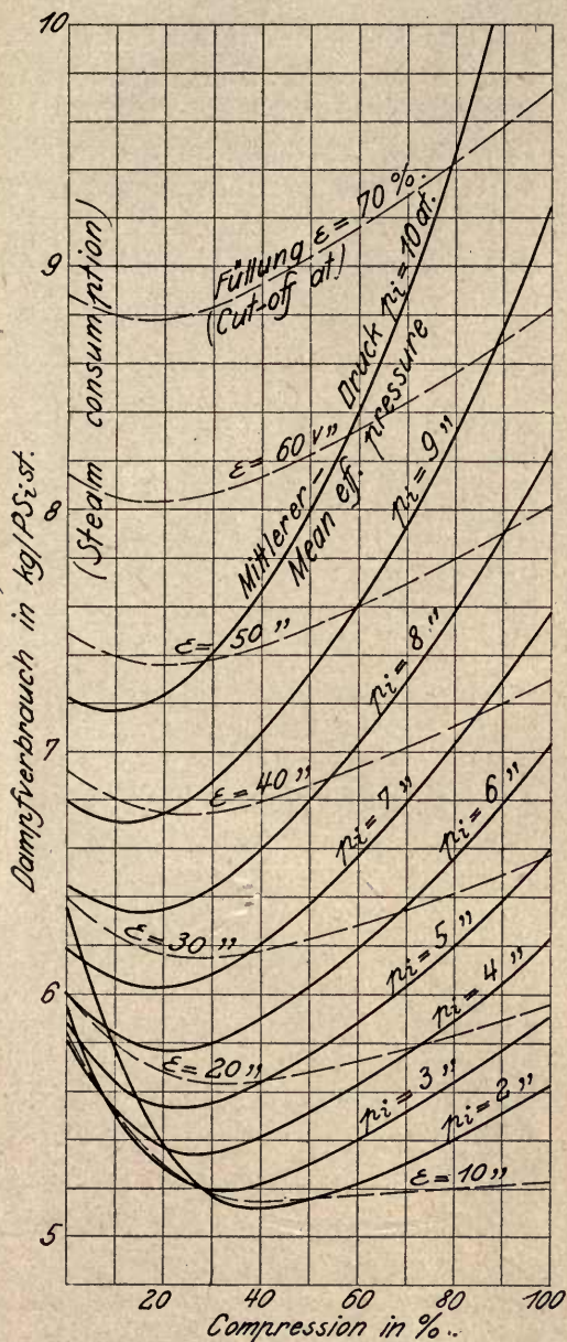
Fig. 13. Superheated steam 300° C, 14 at. abs. Noncondensing, Clearance space 5%.
