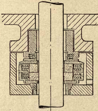
Type A Simplex packing, for steam pressures up to 6 at.
